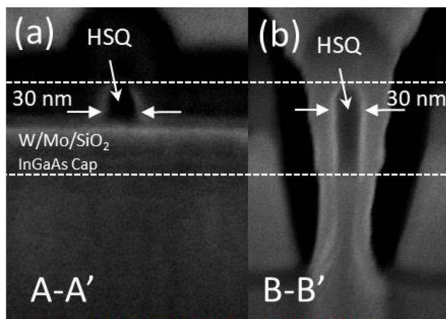
Cross-section of scaled self-aligned InGaAs FinFET
